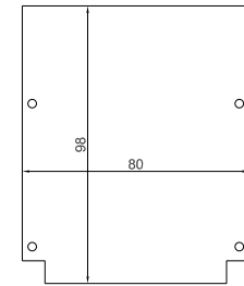
MINIMUM PCB SIZE
