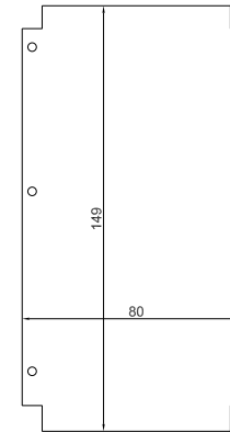
MAXIMUM PCB SIZE
